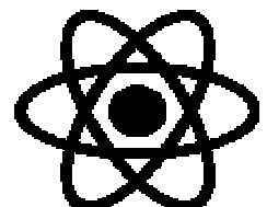
Gamma rays
